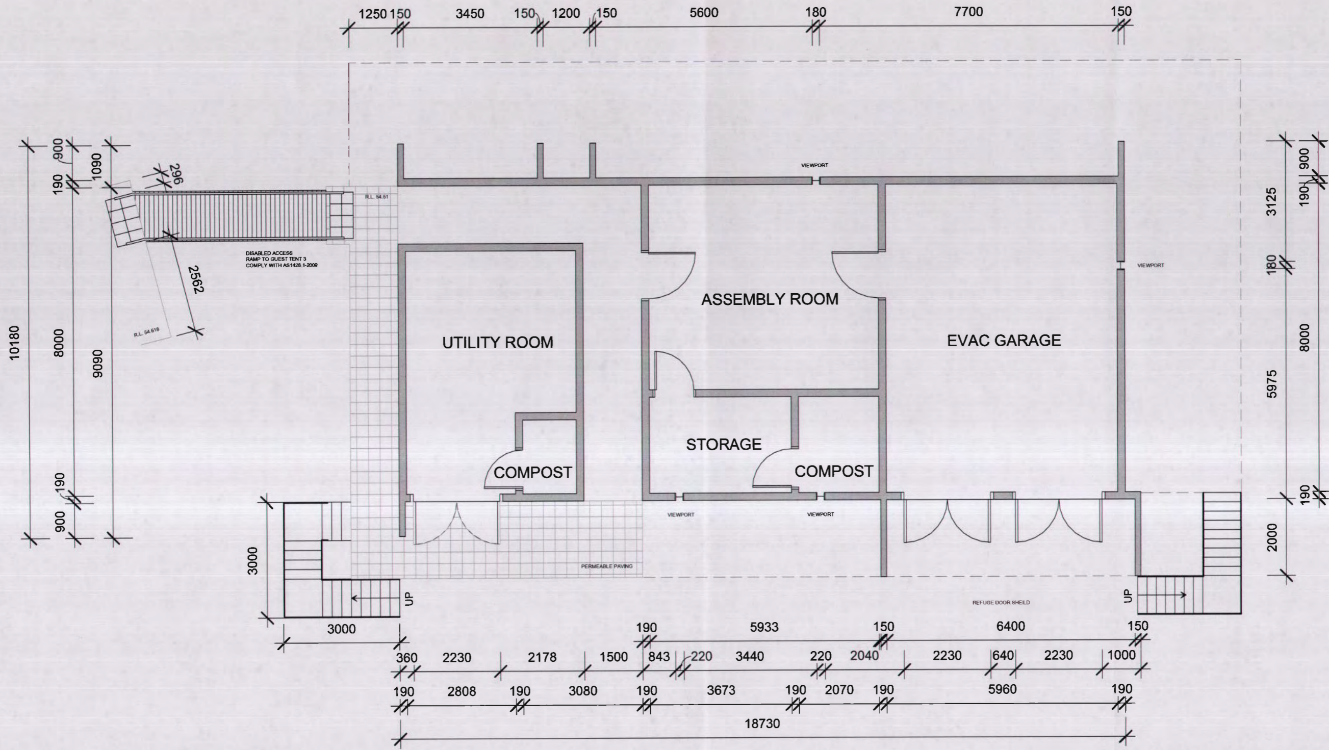
1 GROUND 1 : 100
